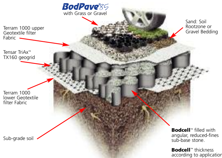
Typical Profile showing various product layers. Not all layers will apply to every application and are optional.
